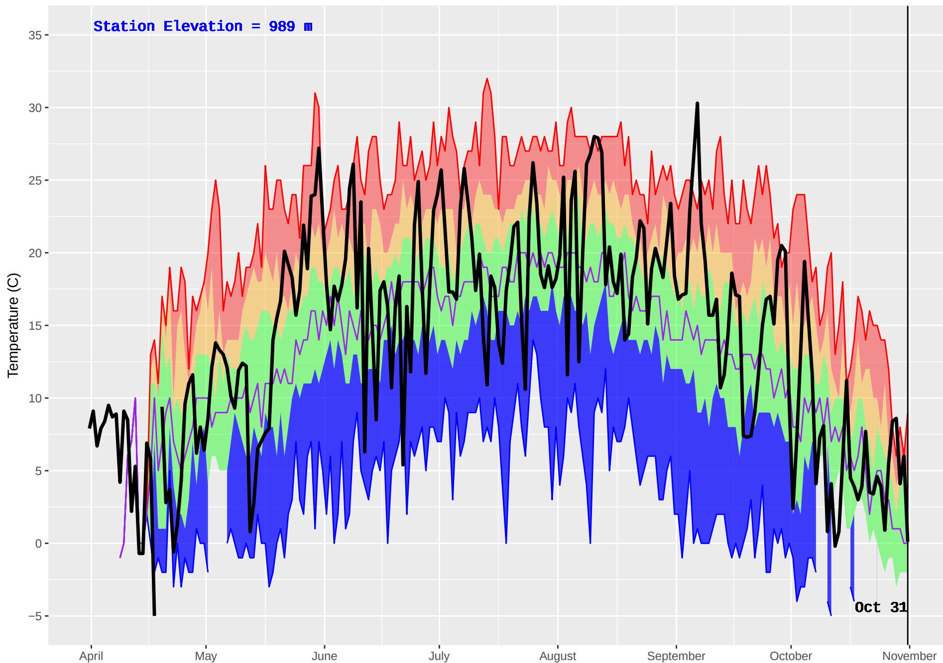
PINK MOUNTAIN (129) : Historical (1983–2016) and Current (2017) Noon Temperature
